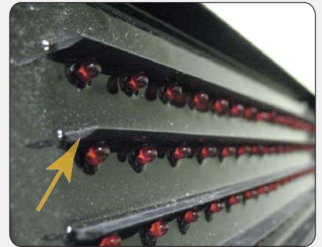
Louvers achieve 6:1 Contrast
